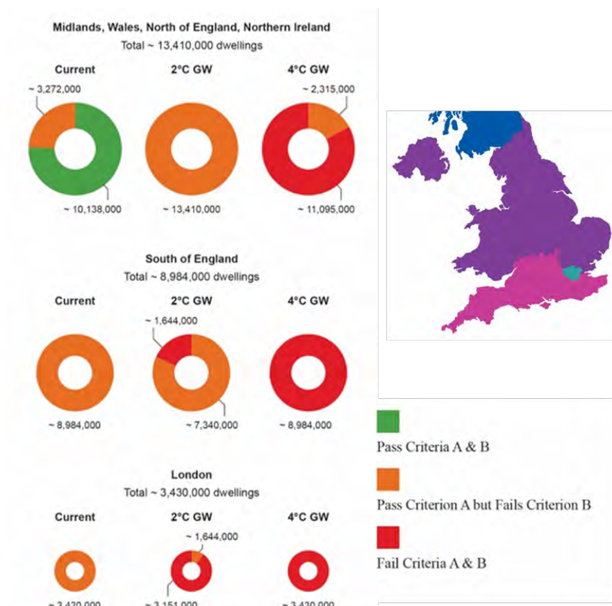
Figure 10.2 Overheating risk across existing homes in England and Northern Ireland according to CIBSE TM59 criteria
